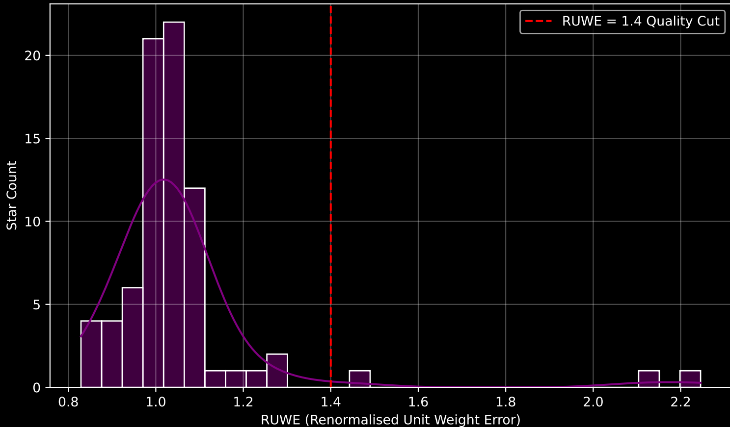
GAPOGEE DR17 Field [LMC18] RUWE Distribution (n= 77)
