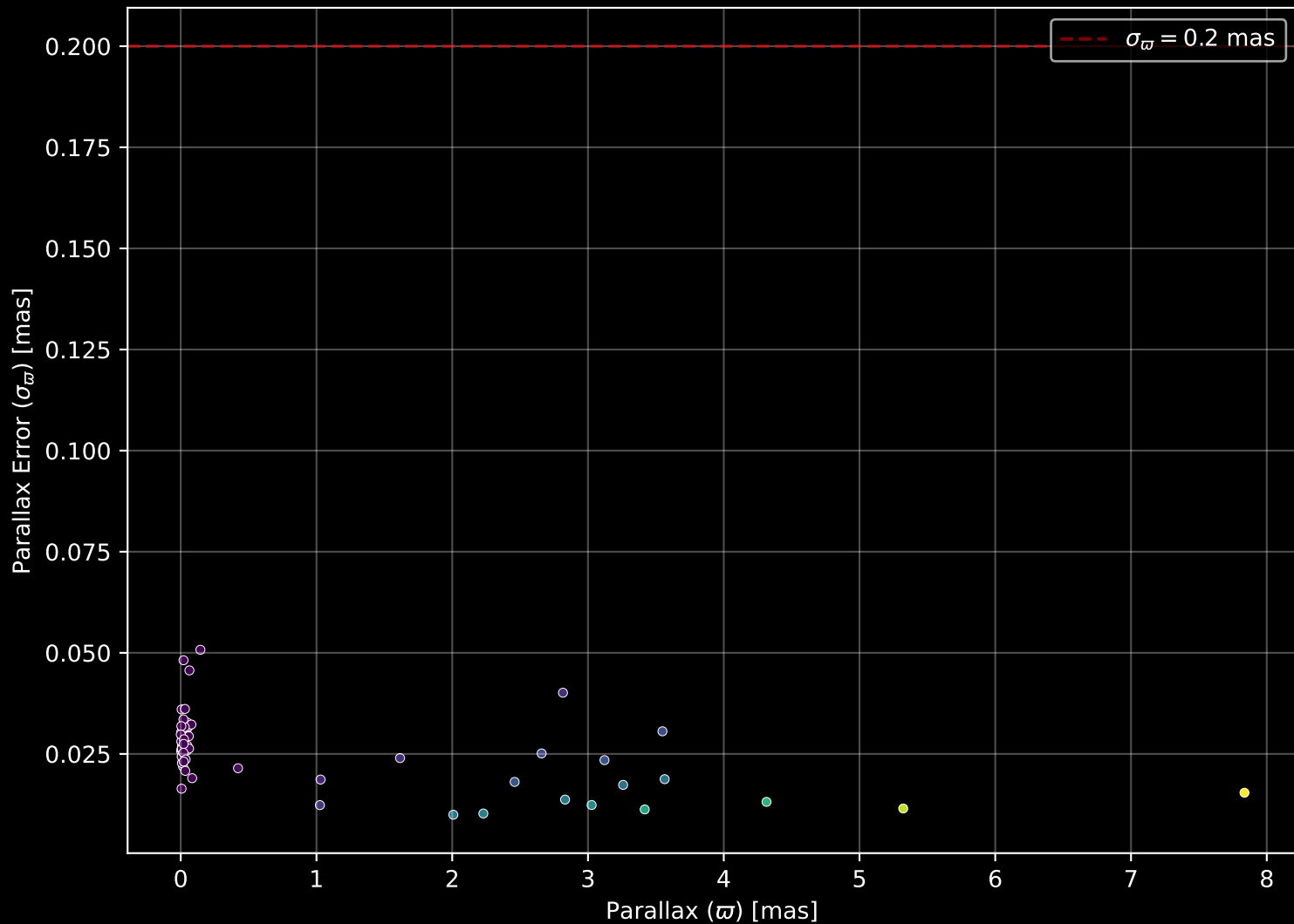
APOGEE DR17 Field: [LMC18] Parallax Quality (n= 77)
